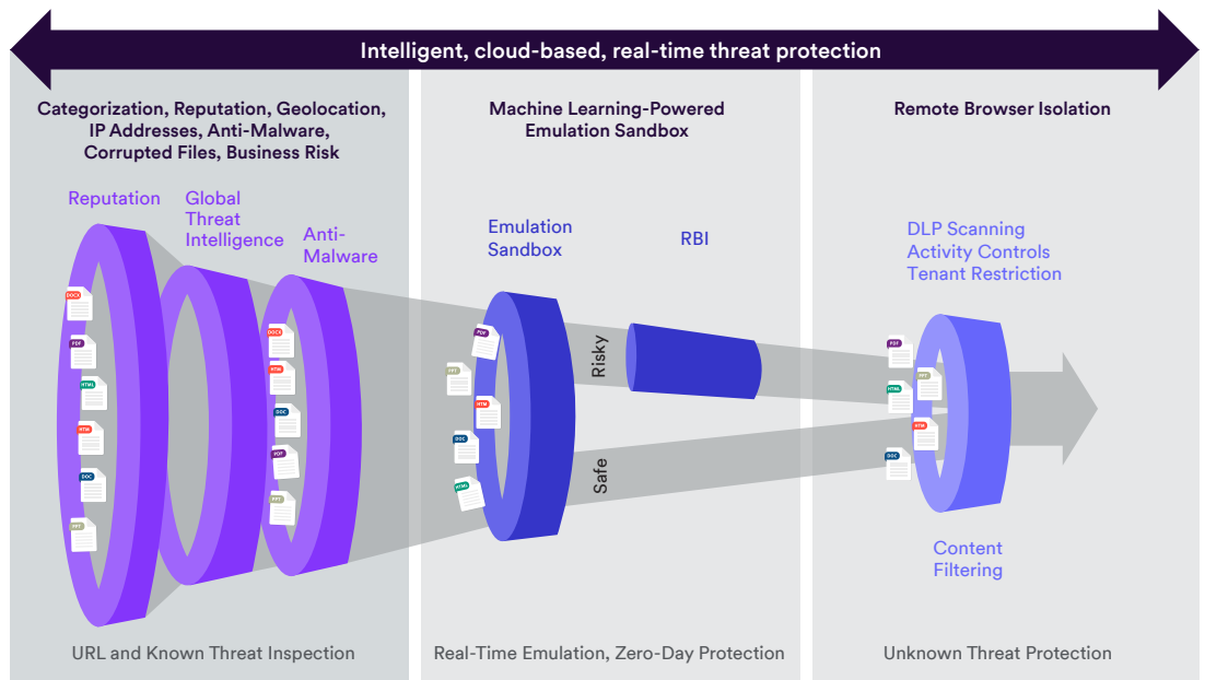
Figure 3. Skyhigh Security Service Edge Integrated Threat Protection
